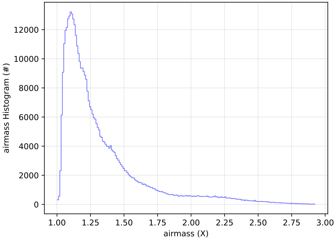
too_elab_r128_d3_ugrizy_v3.4_10yrs All sky z band: airmass Histogram
