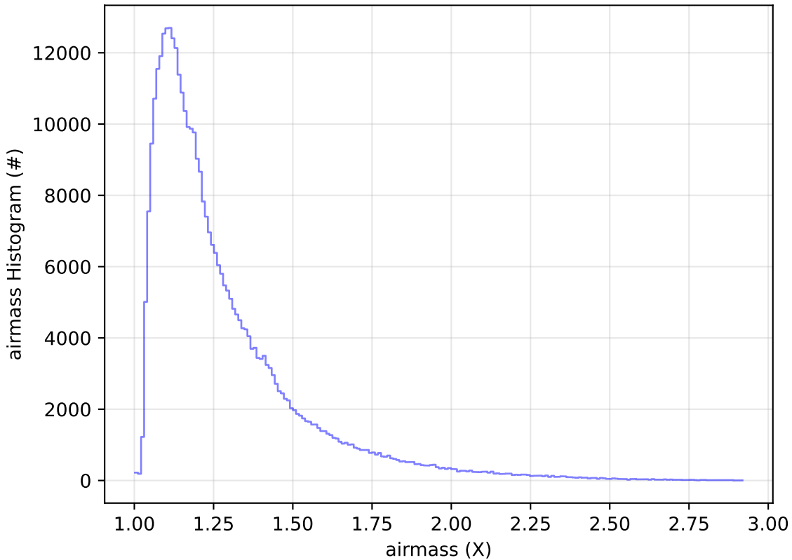
too_elab_r128_d3_ugrizy_v3.4_10yrs All sky y band: airmass Histogram
