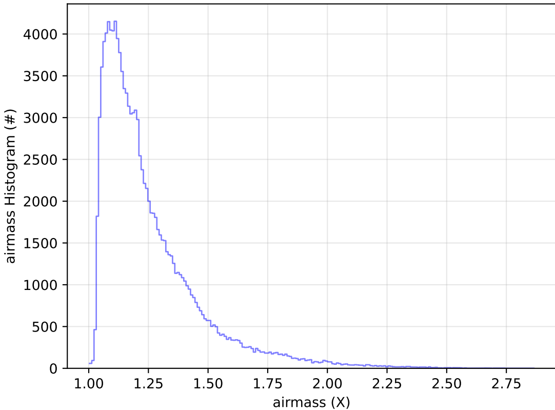
too_elab_r128_d3_ugrizy_v3.4_10yrs All sky u band: airmass Histogram
