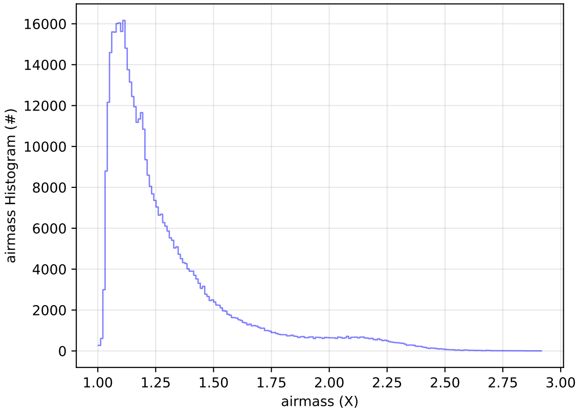
too_elab_r128_d3_ugrizy_v3.4_10yrs All sky r band: airmass Histogram
