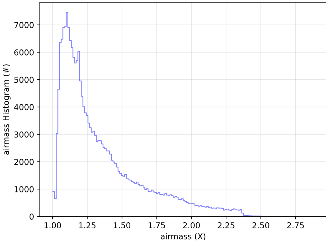
too_elab_r128_d3_ugrizy_v3.4_10yrs All sky g band: airmass Histogram
