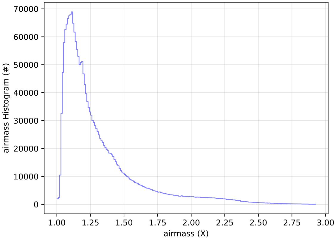
too_elab_r128_d3_ugrizy_v3.4_10yrs All sky all bands: airmass Histogram
