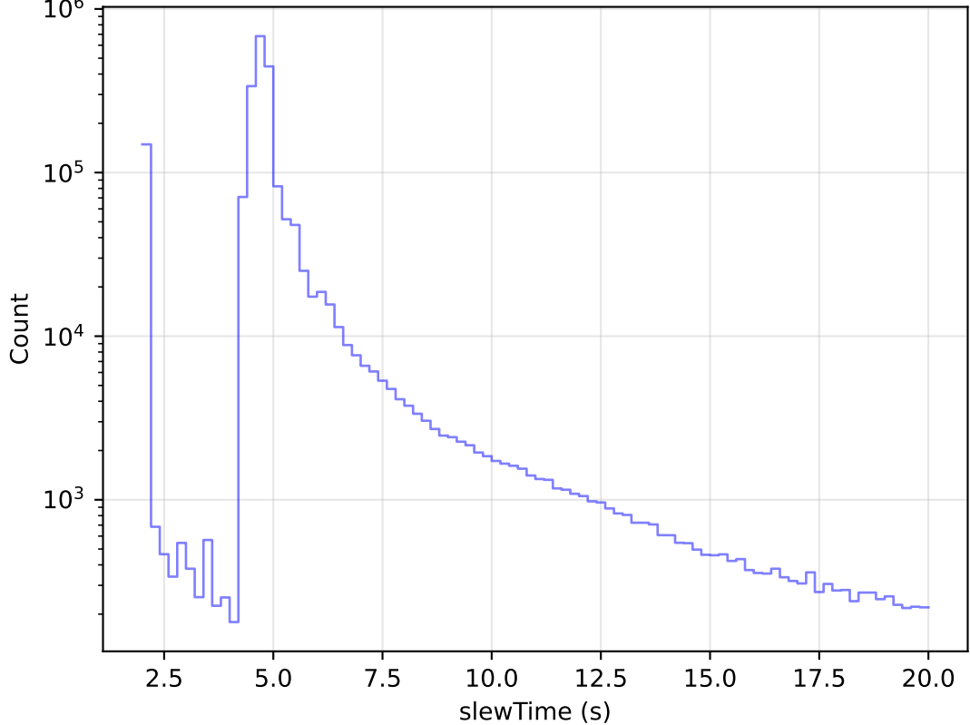
too_elab_r128_d3_ugrizy_v3.4_10yrs All visits: Zoom Slew Time Histogram
