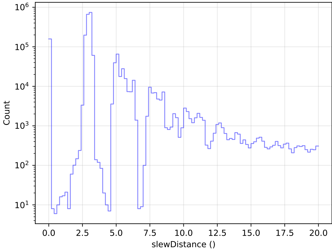
too_elab_r128_d3_ugrizy_v3.4_10yrs All visits: Zoom Slew Distance Histogram
