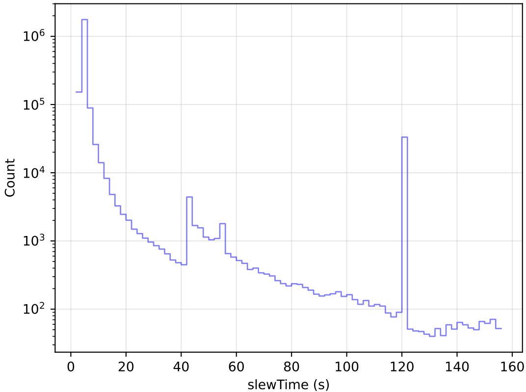
too_elab_r128_d3_ugrizy_v3.4_10yrs All visits: Slew Time Histogram
