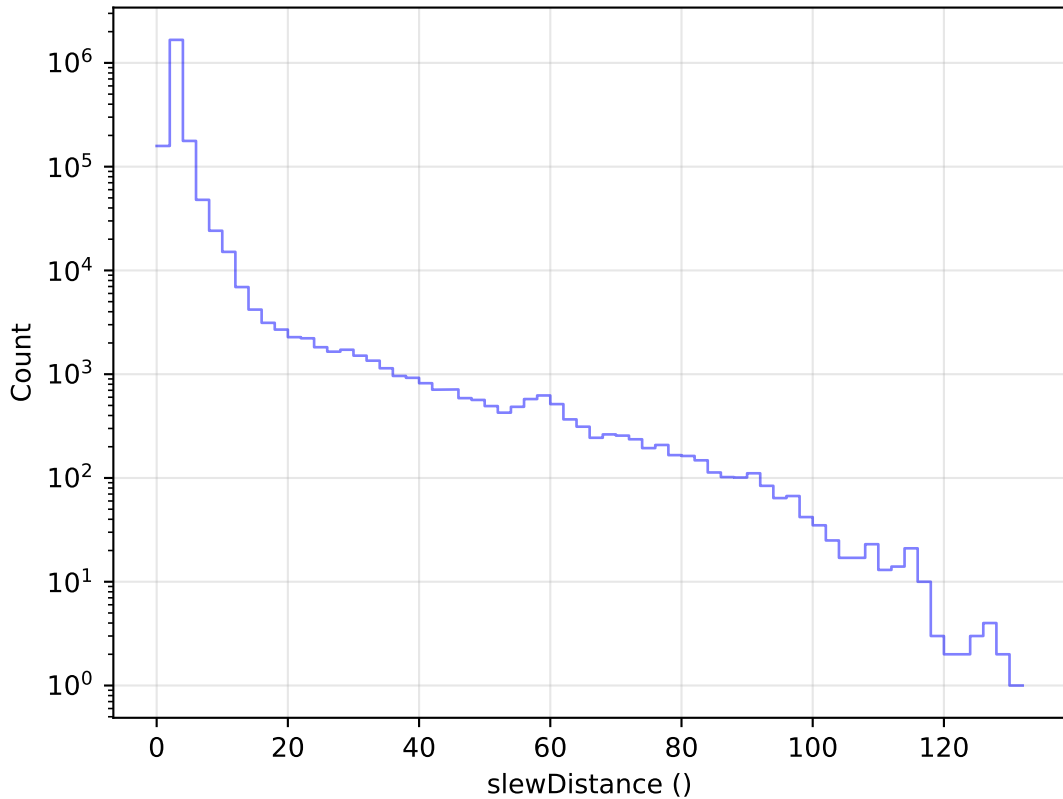
too_elab_r128_d3_ugrizy_v3.4_10yrs All visits: Slew Distance Histogram
