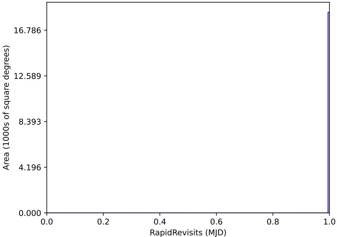
too_elab_r128_d3_ugrizy_v3.4_10yrs WFD: RapidRevisits
