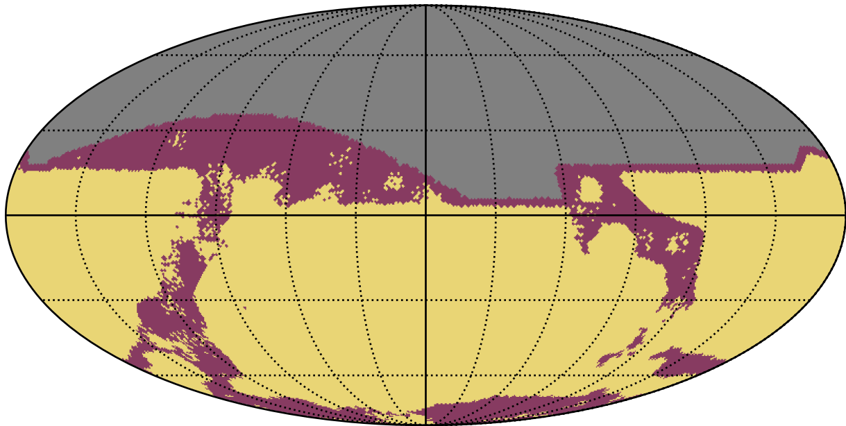
too_elab_r128_d3_ugrizy_v3.4_10yrs All sky: RapidRevisits
