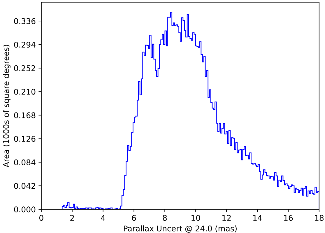
too_elab_r128_d3_ugrizyv3.4_10yrs All sky: Parallax Uncert @ 24.0
