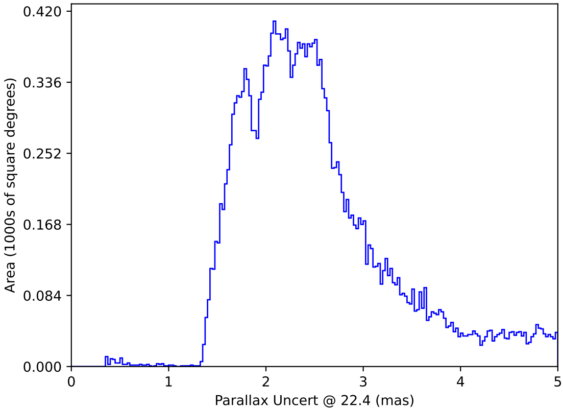
too_elab_r128_d3_ugrizy_v3.4_10yrs All sky: Parallax Uncert @ 22.4
