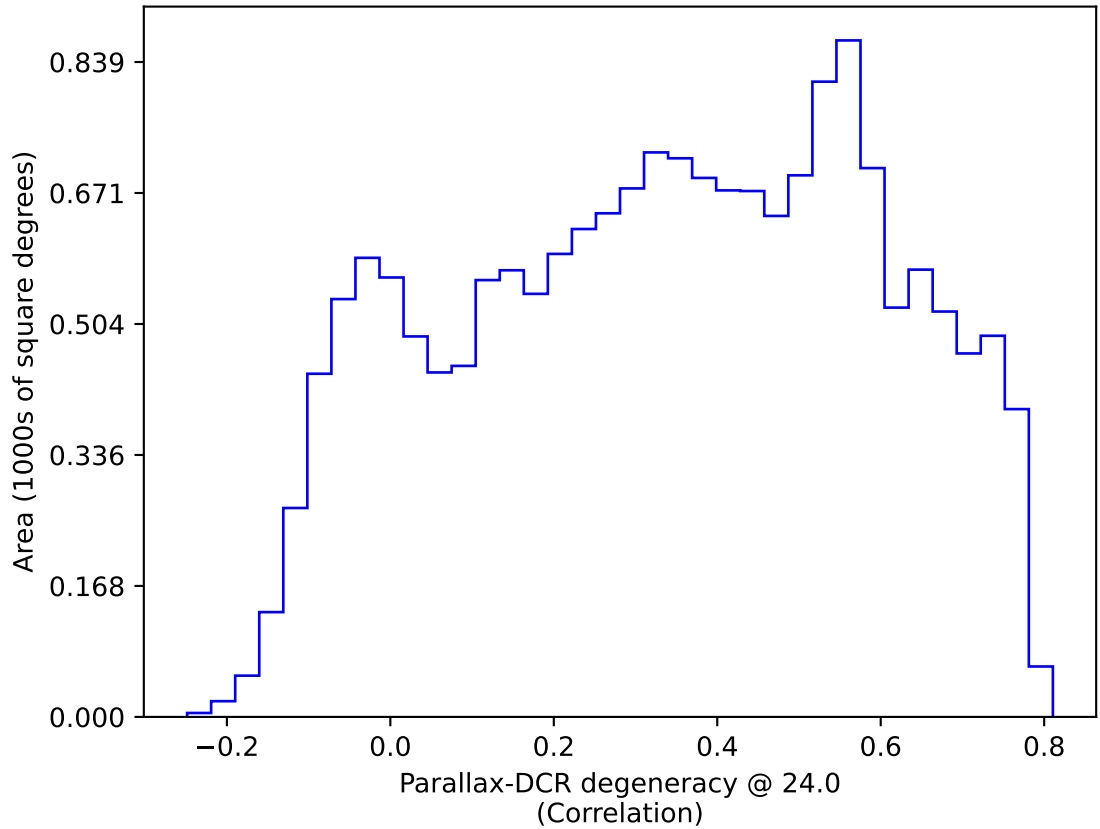
too_elab_r128_d3_ugrizy_v3.4_10yrs WFD: Parallax-DCR degeneracy @ 24.0
