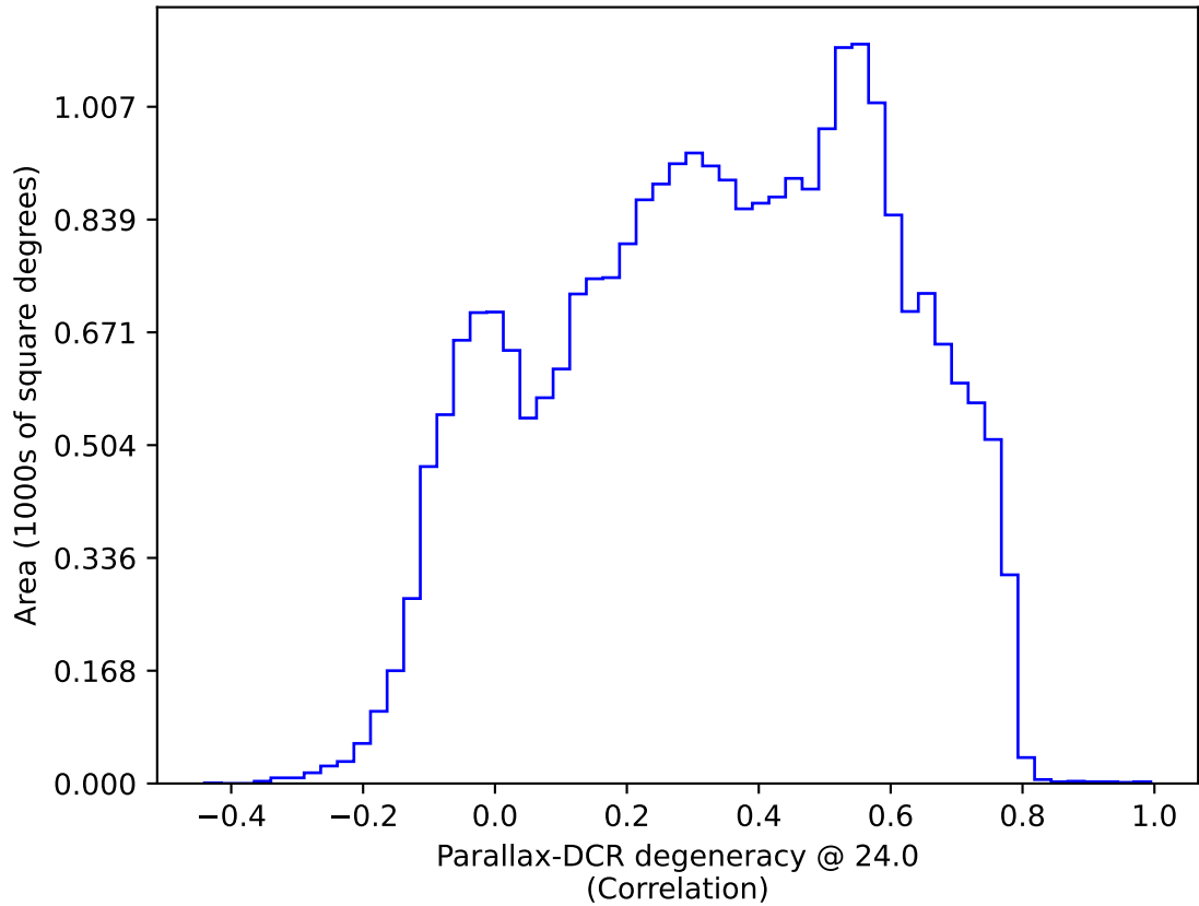
too_elab_r128_d3_ugrizy_v3.4_10yrs All sky: Parallax-DCR degeneracy @ 24.0
