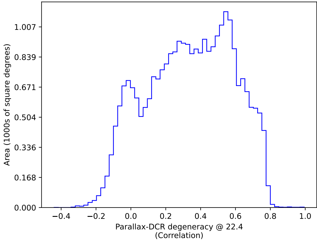
too_elab_r128_d3_ugrizy_v3.4_10yrs All sky: Parallax-DCR degeneracy @ 22.4
