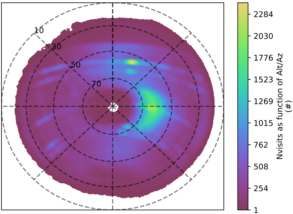
too_elab_r128_d3_ugrizy_v3.4_10yrs z band: Nvisits as function of Alt/Az
