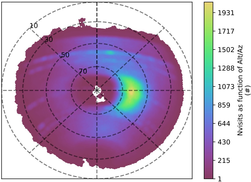
too_elab_r128_d3_ugrizy_v3.4_10yrs y band: Nvisits as function of Alt/Az
