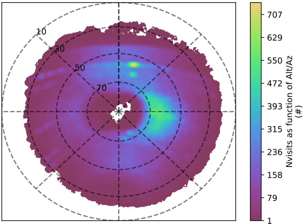
too_elab_r128_d3_ugrizy_v3.4_10yrs u band: Nvisits as function of Alt/Az
