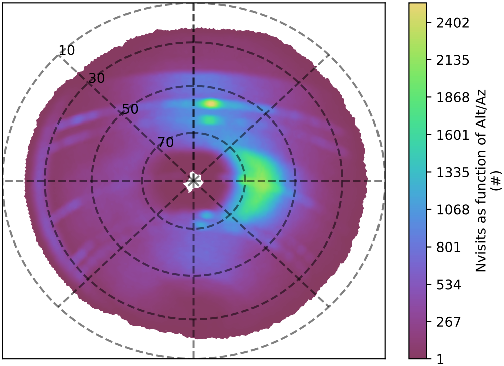
too_elab_r128_d3_ugrizy_v3.4_10yrs r band: Nvisits as function of Alt/Az
