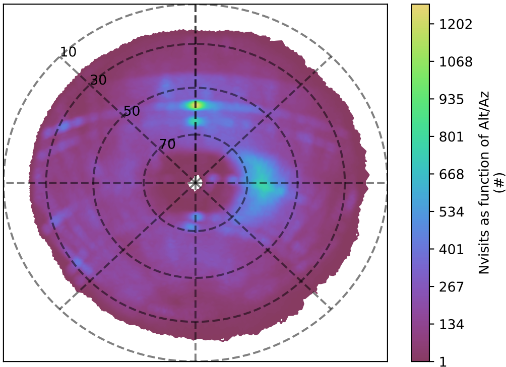
too_elab_r128_d3_ugrizy_v3.4_10yrs g band: Nvisits as function of Alt/Az
