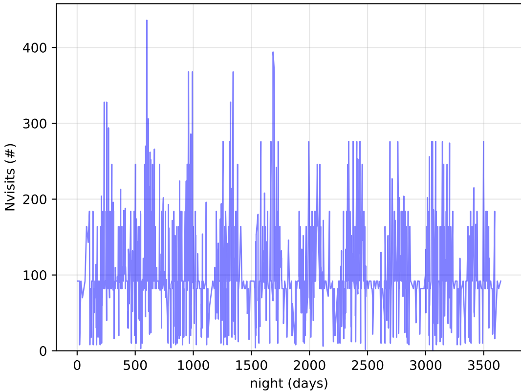
too_elab_r128_d3_ugrizy_v3.4_10yrs DDF: Nvisits
