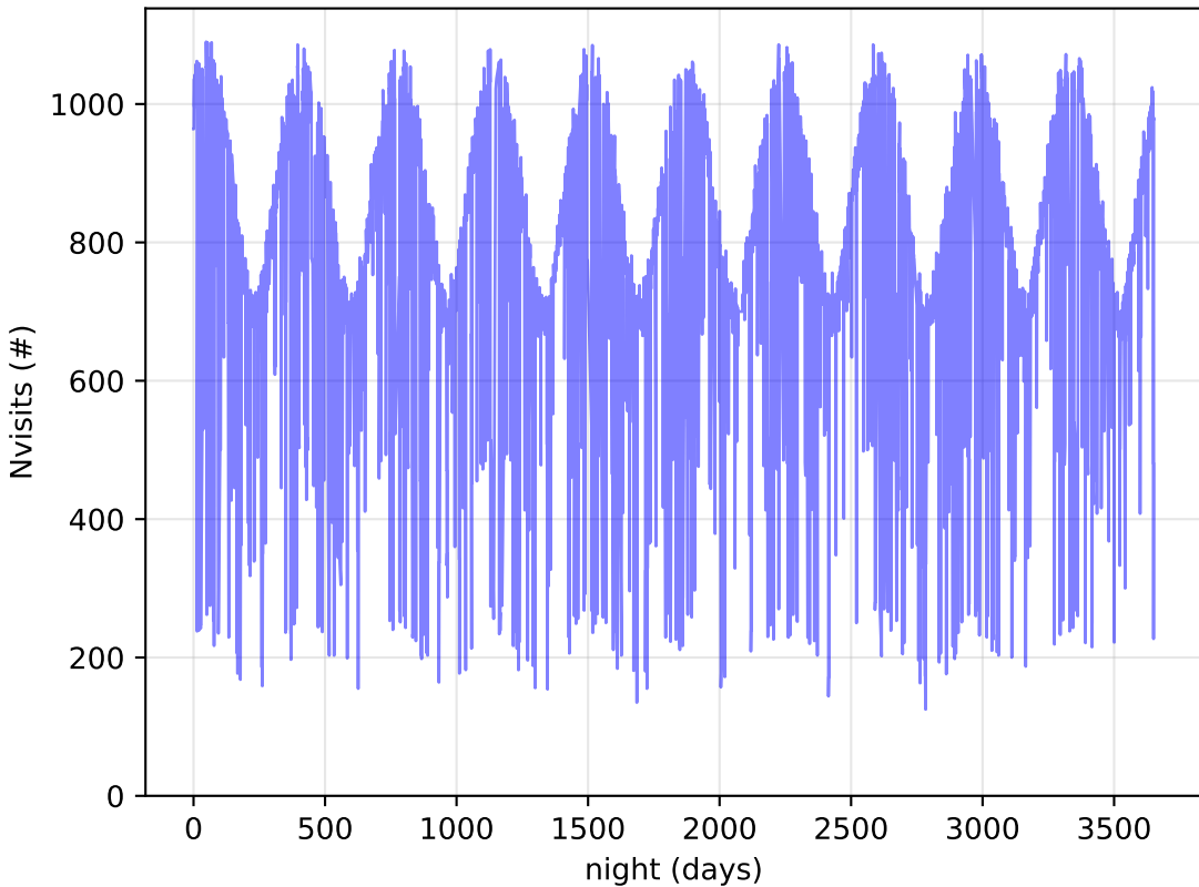
too_elab_r128_d3_ugrizy_v3.4_10yrs All visits: Nvisits
