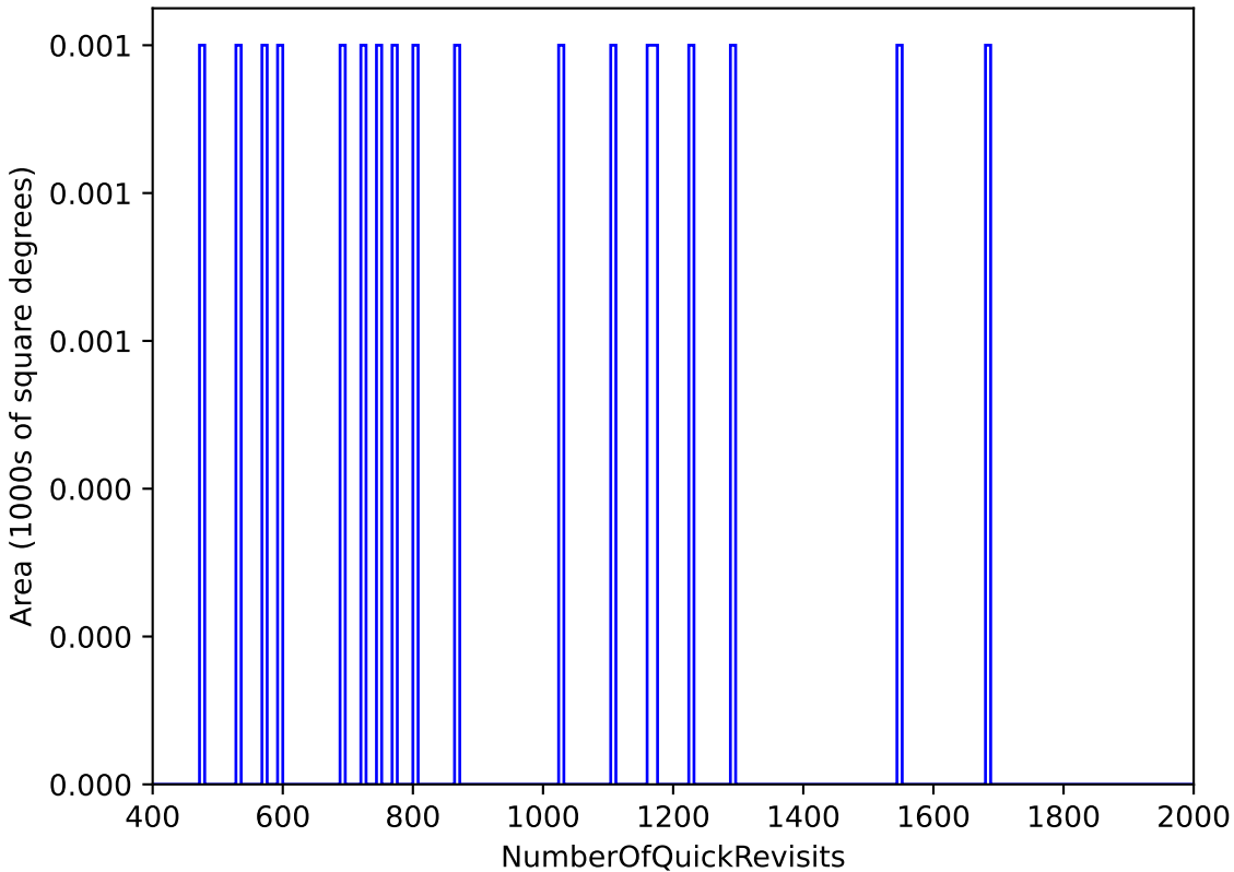
too_elab_r128_d3_ugrizy_v3.4_10yrs WFD: NumberOfQuickRevisits
