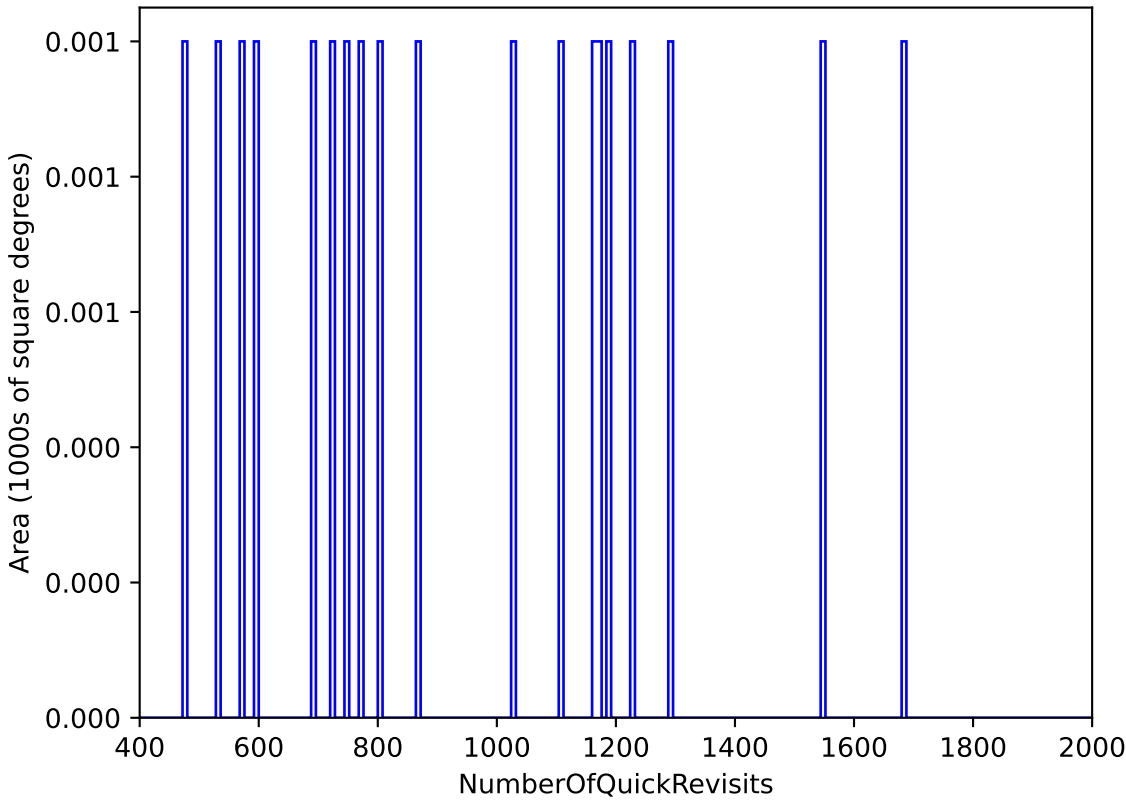
too_elab_r128_d3_ugrizy_v3.4_10yrs All sky: NumberOfQuickRevisits
