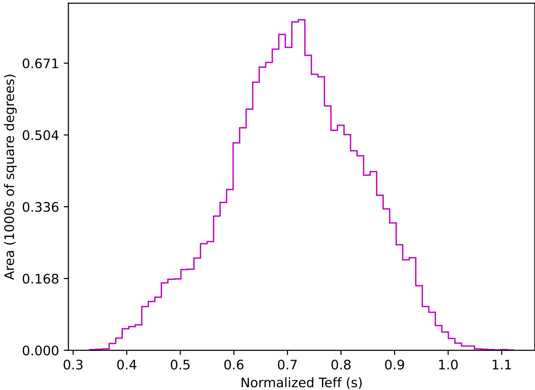
too_elab_r128_d3_ugrizy_v3.4_10yrs WFD z band: Normalized Teff
