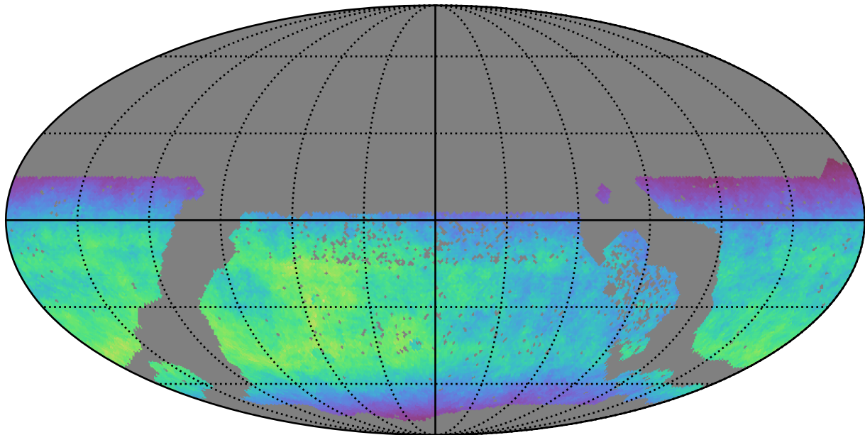
too_elab_r128_d3_ugrizy_v3.4_10yrs WFD y band: Normalized Teff
