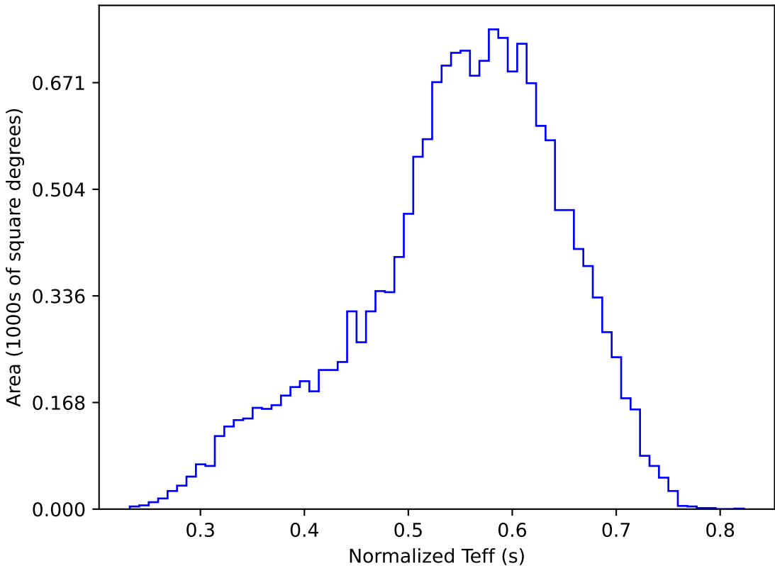
too_elab_r128_d3_ugrizy_v3.4_10yrs WFD y band: Normalized Teff
