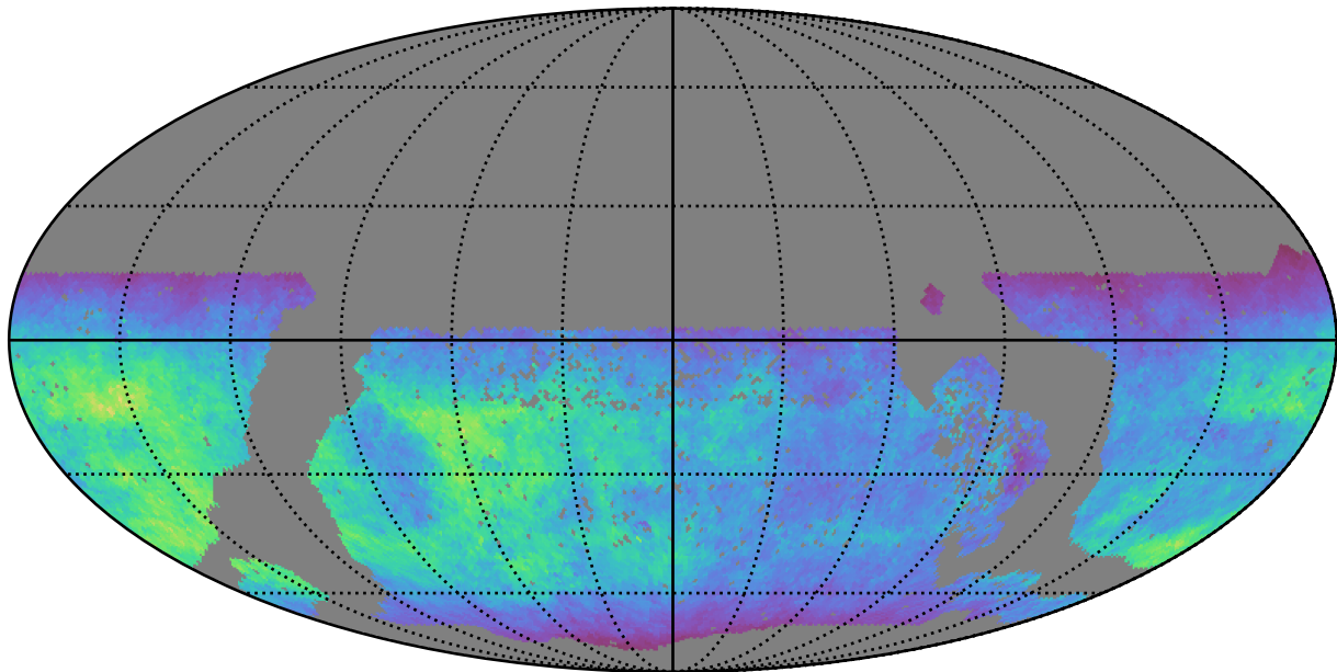
too_elab_r128_d3_ugrizy_v3.4_10yrs WFD u band: Normalized Teff
