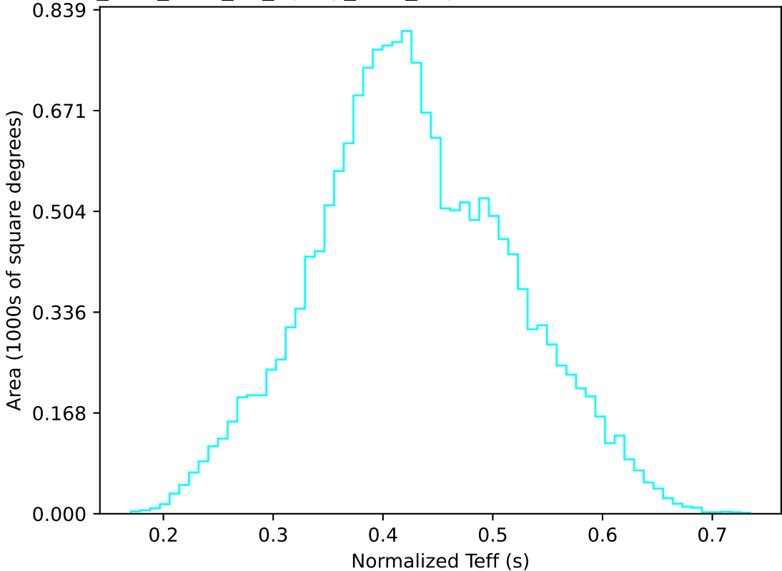
too_elab_r128_d3_ugrizy_v3.4_10yrs WFD u band: Normalized Teff
