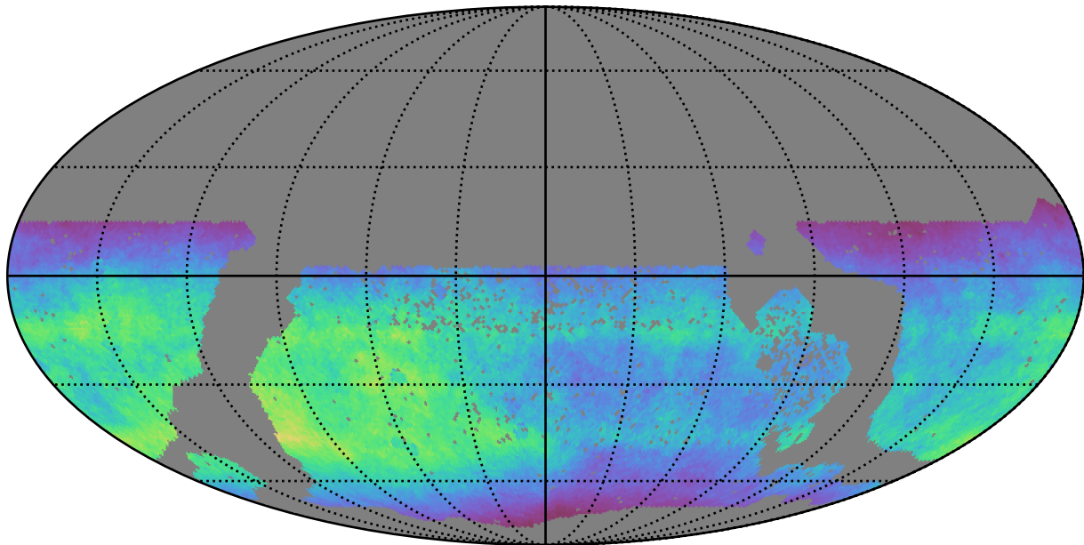
too_elab_r128_d3_ugrizy_v3.4_10yrs WFD i band: Normalized Teff
