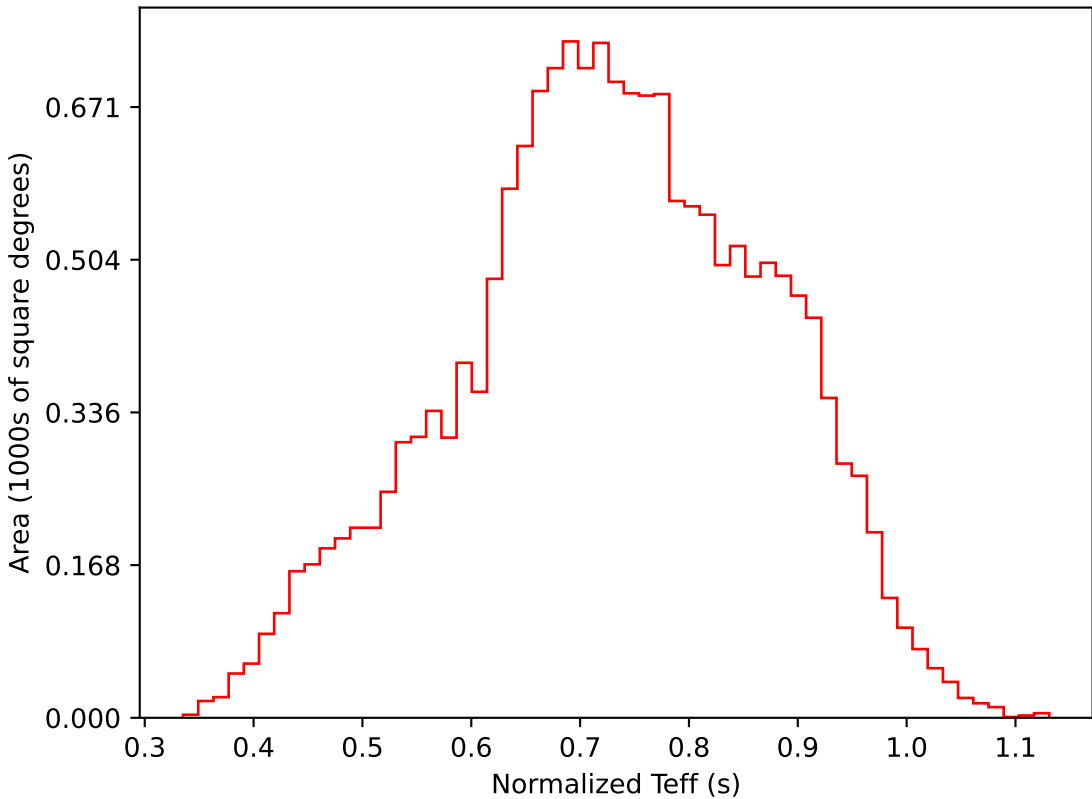
too_elab_r128_d3_ugrizy_v3.4_10yrs WFD i band: Normalized Teff
