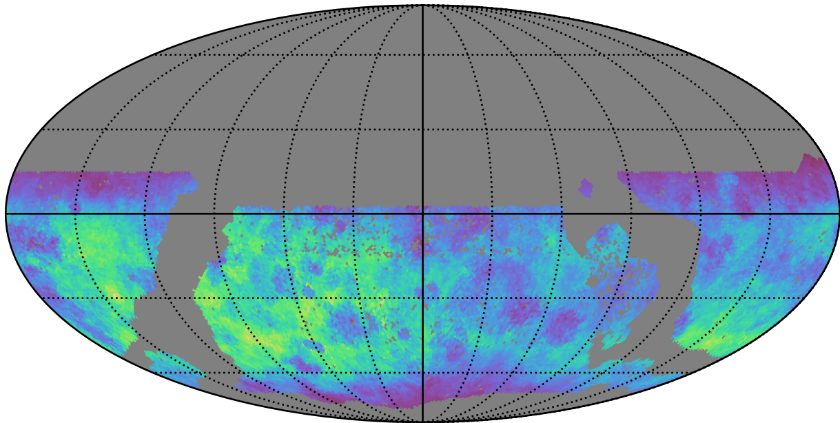
too_elab_r128_d3_ugrizy_v3.4_10yrs WFD g band: Normalized Teff
