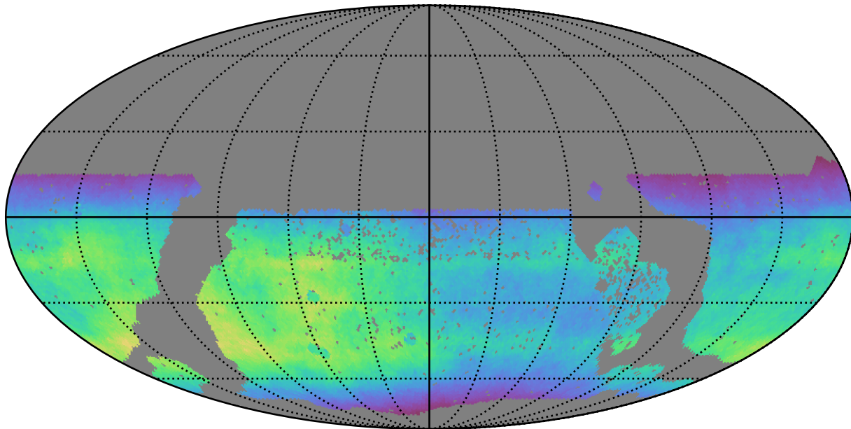
too_elab_r128_d3_ugrizy_v3.4_10yrs WFD all bands: Normalized Teff
