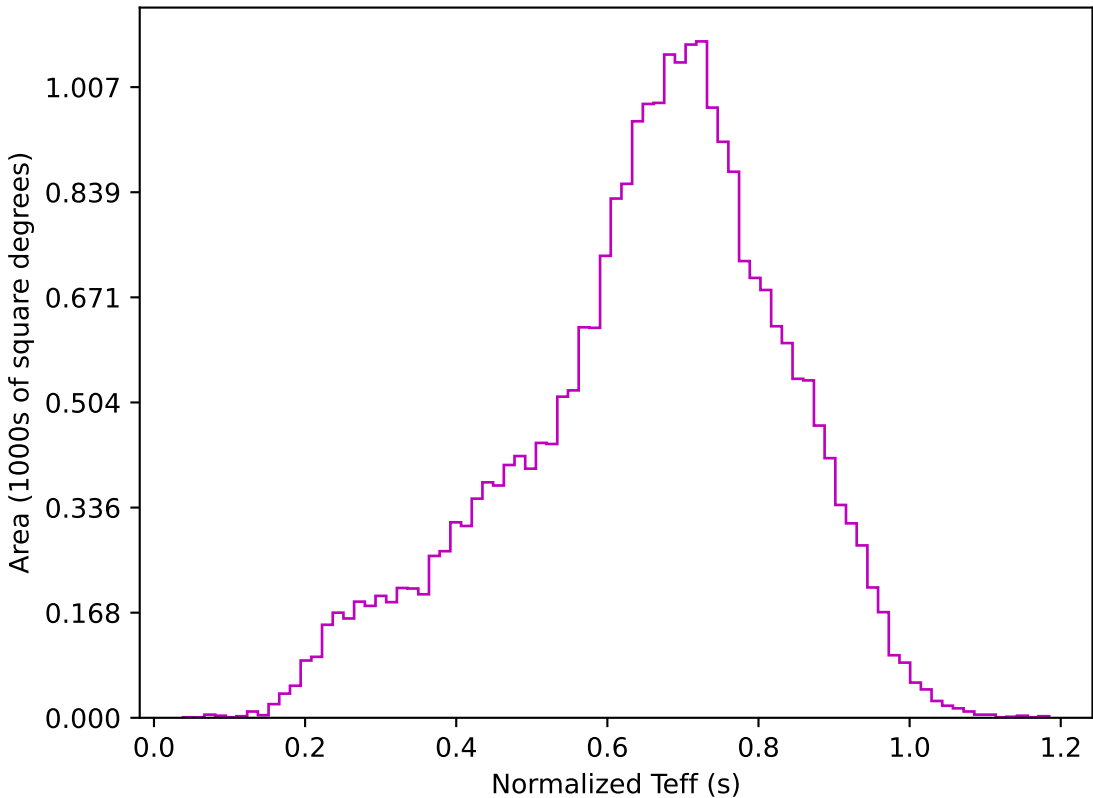
too_elab_r128_d3_ugrizy_v3.4_10yrs All sky z band: Normalized Teff
