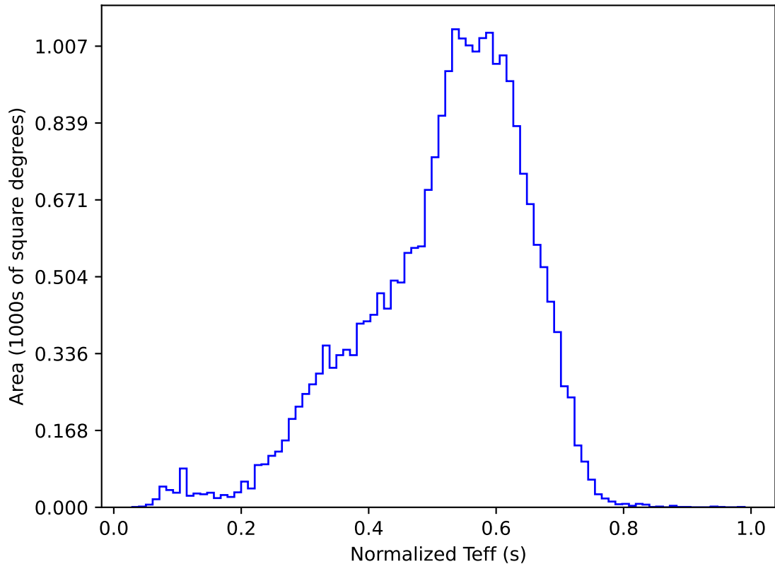
too_elab_r128_d3_ugrizy_v3.4_10yrs All sky y band: Normalized Teff
