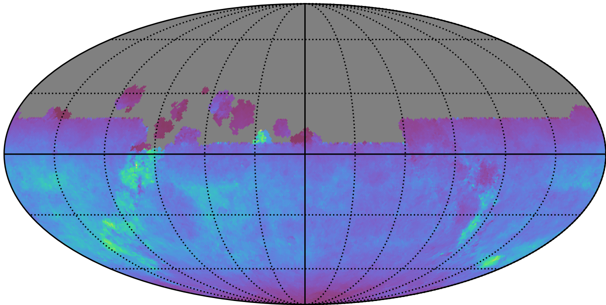
too_elab_r128_d3_ugrizy_v3.4_10yrs All sky u band: Normalized Teff
