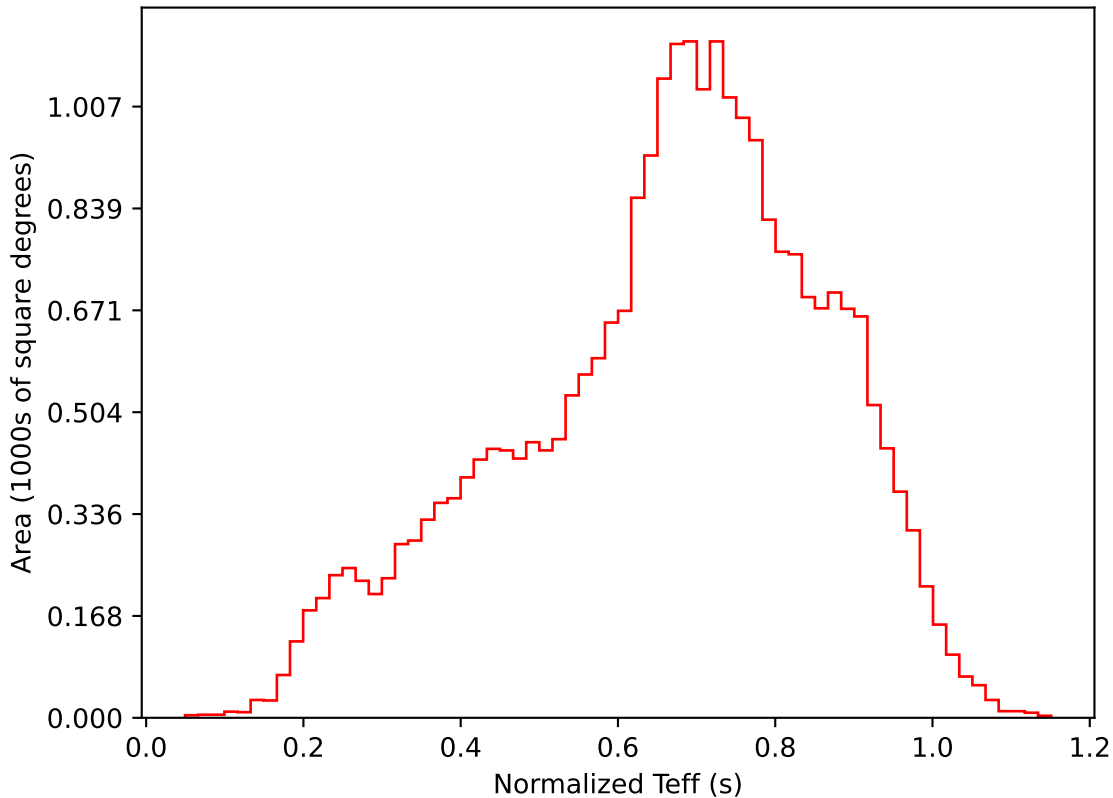
too_elab_r128_d3_ugrizy_v3.4_10yrs All sky i band: Normalized Teff
