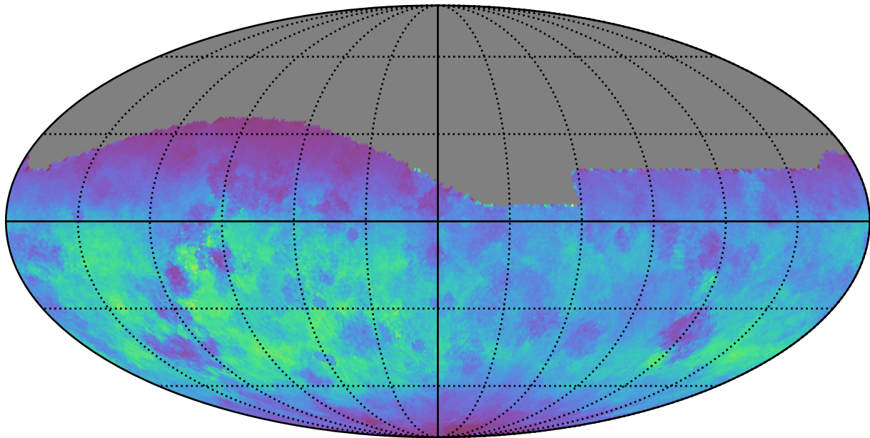
too_elab_r128_d3_ugrizy_v3.4_10yrs All sky g band: Normalized Teff
