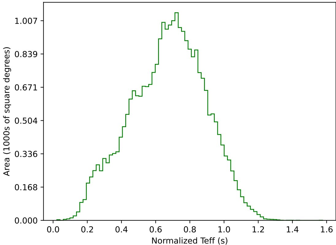
too_elab_r128_d3_ugrizy_v3.4_10yrs All sky g band: Normalized Teff
