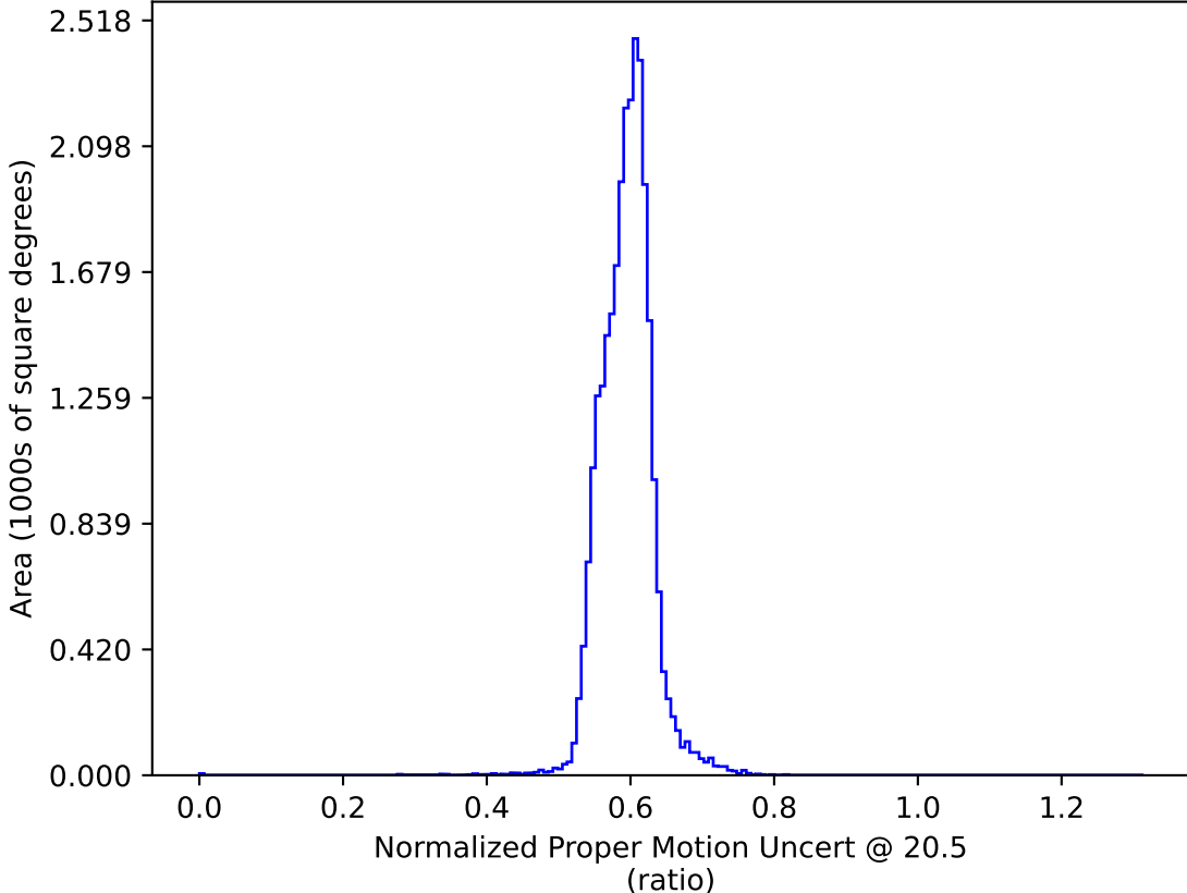
too_elab_r128_d3_ugrizy_v3.4_10yrs All sky: Normalized Proper Motion Uncert @ 20.5
