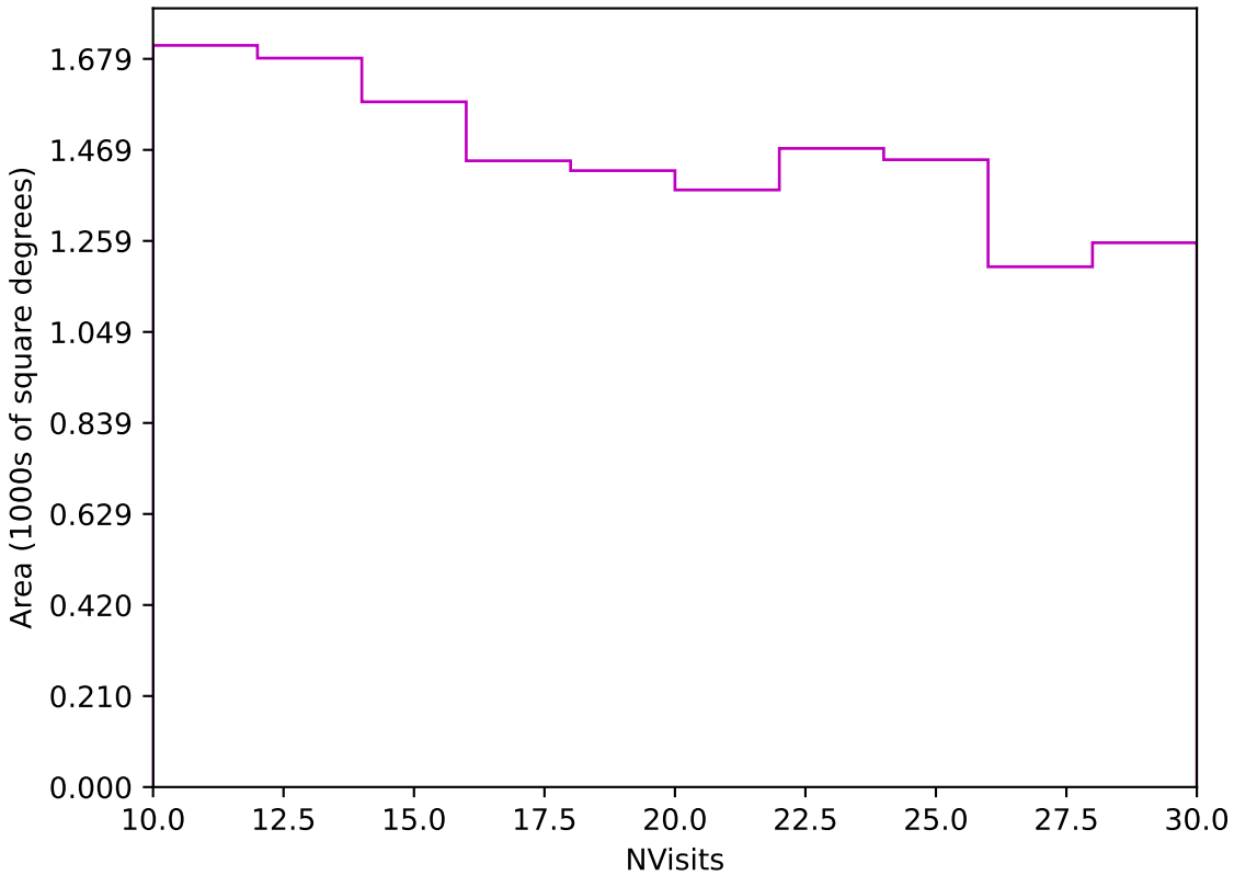
too_elab_r128_d3_ugrizy_v3.4_10yrs Yr 3-4 z band: NVisits
