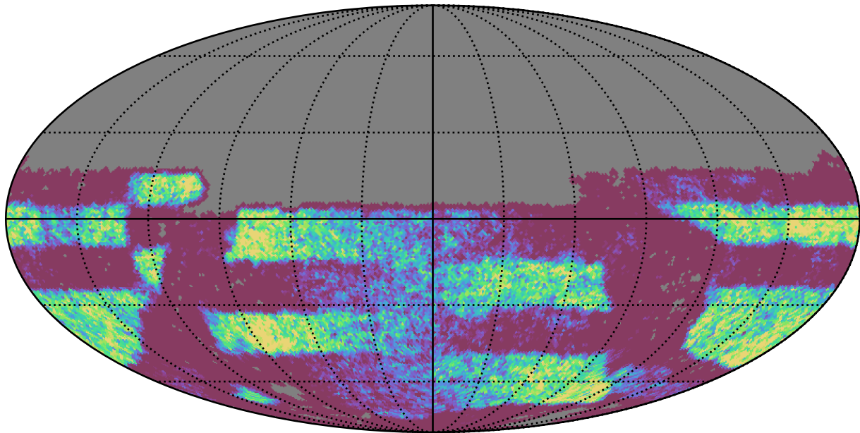
too_elab_r128_d3_ugrizy_v3.4_10yrs Yr 3-4 y band: NVisits
