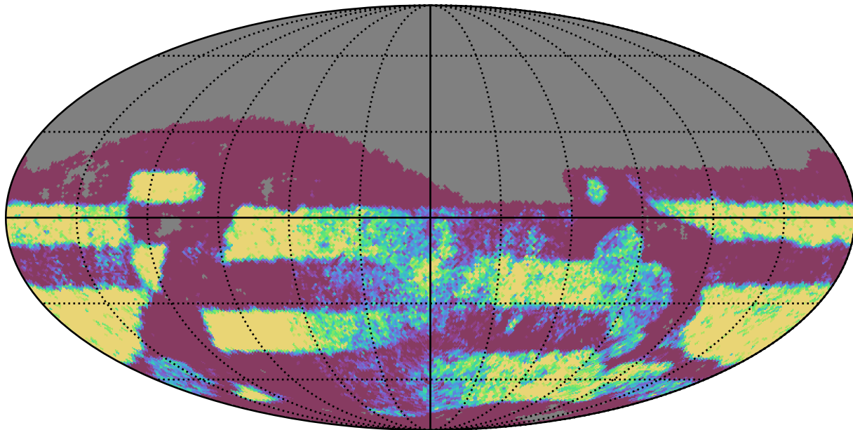
too_elab_r128_d3_ugrizy_v3.4_10yrs Yr 3-4 r band: NVisits
