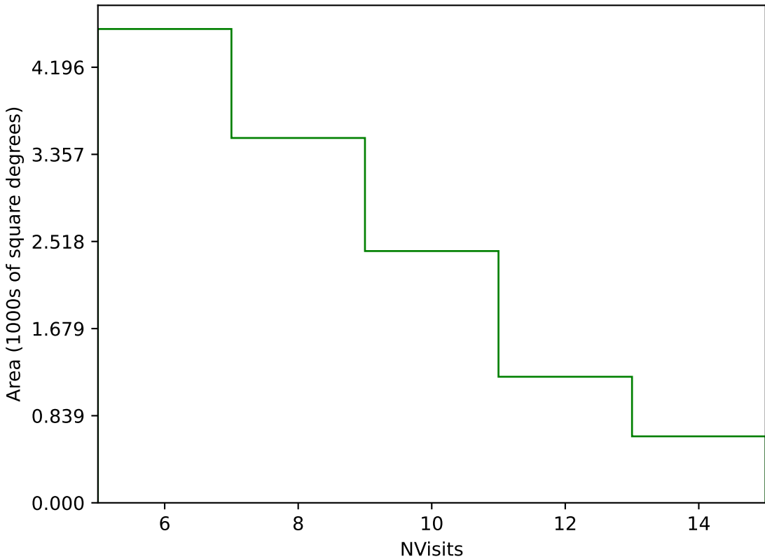
too_elab_r128_d3_ugrizy_v3.4_10yrs Yr 3-4 g band: NVisits
