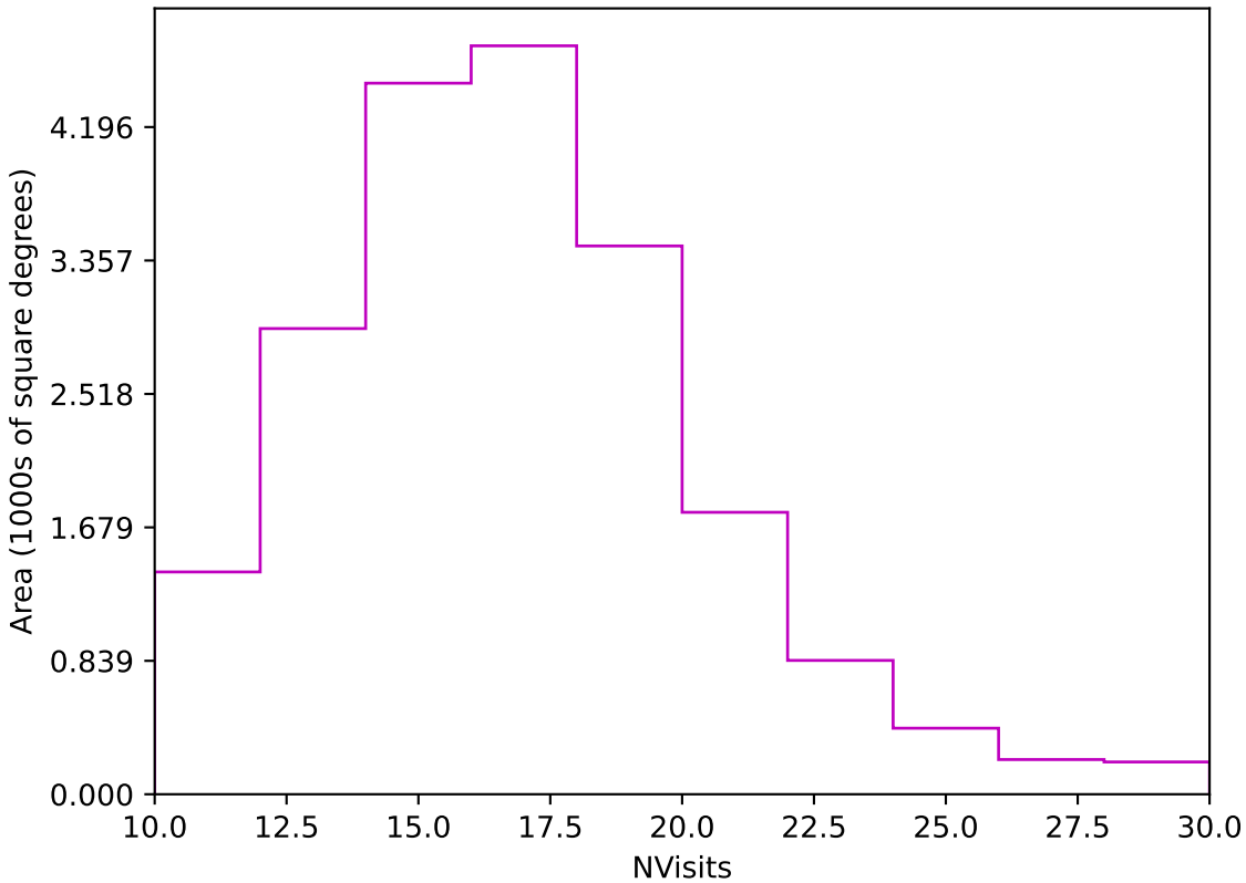
too_elab_r128_d3_ugrizy_v3.4_10yrs Yr 1 z band: NVisits
