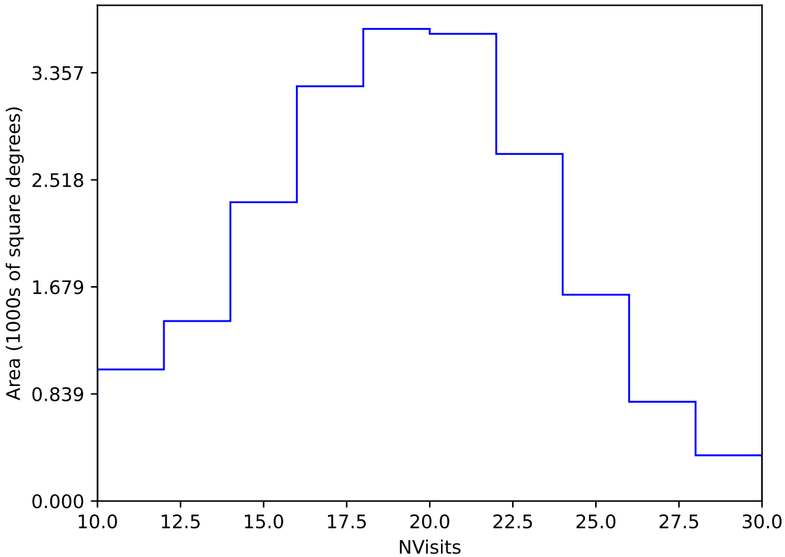
too_elab_r128_d3_ugrizy_v3.4_10yrs Yr 1 y band: NVisits
