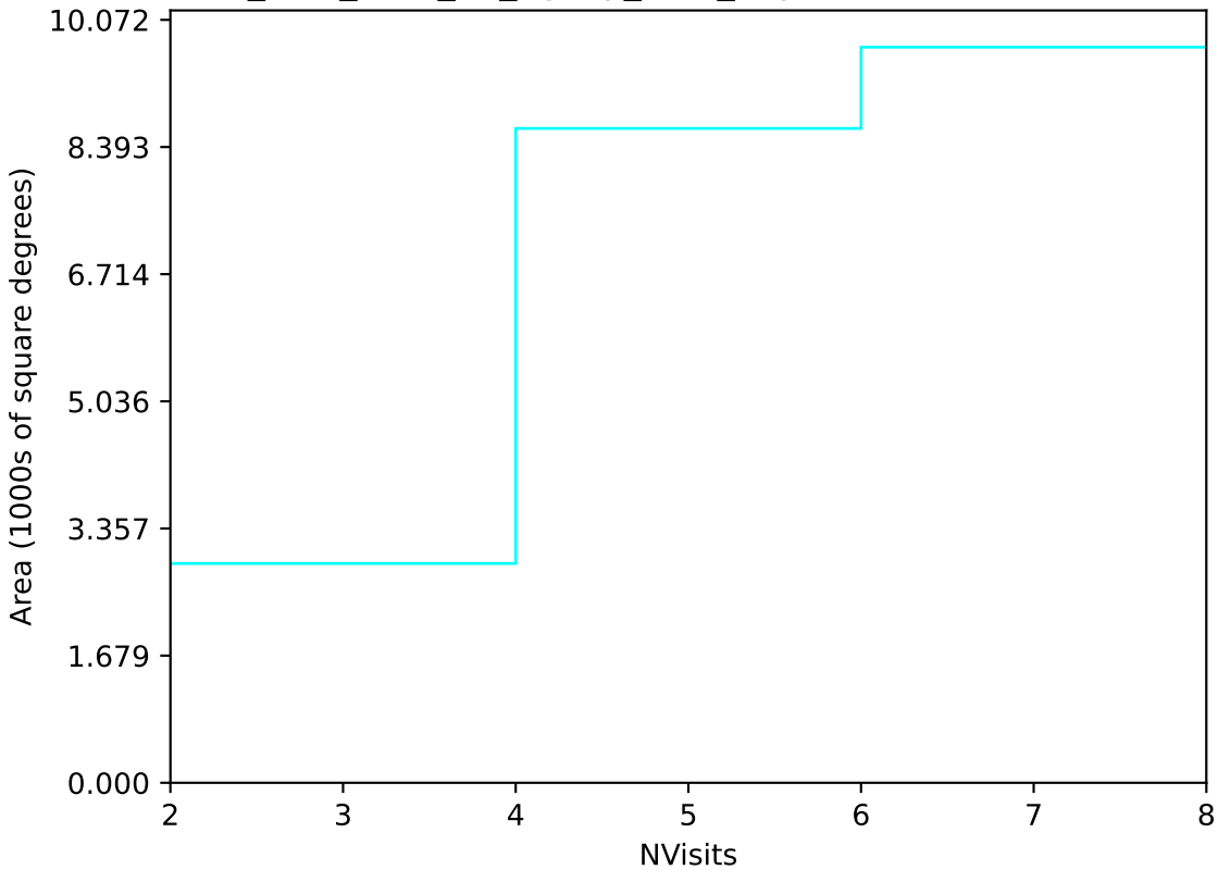
too_elab_r128_d3_ugrizy_v3.4_10yrs Yr 1 u band: NVisits
