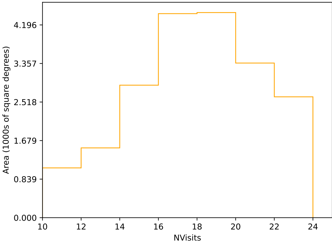
too_elab_r128_d3_ugrizy_v3.4_10yrs Yr 1 r band: NVisits
